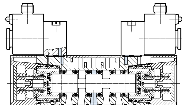
Sectional view MDH-5/3...
