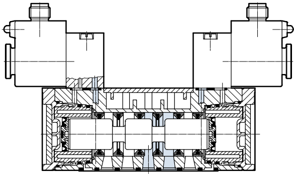
Sectional view JMDH-5/2- ..., JMDDH-5/2- ...
