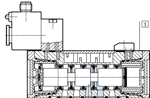
Sectional view MDH-5/3...
